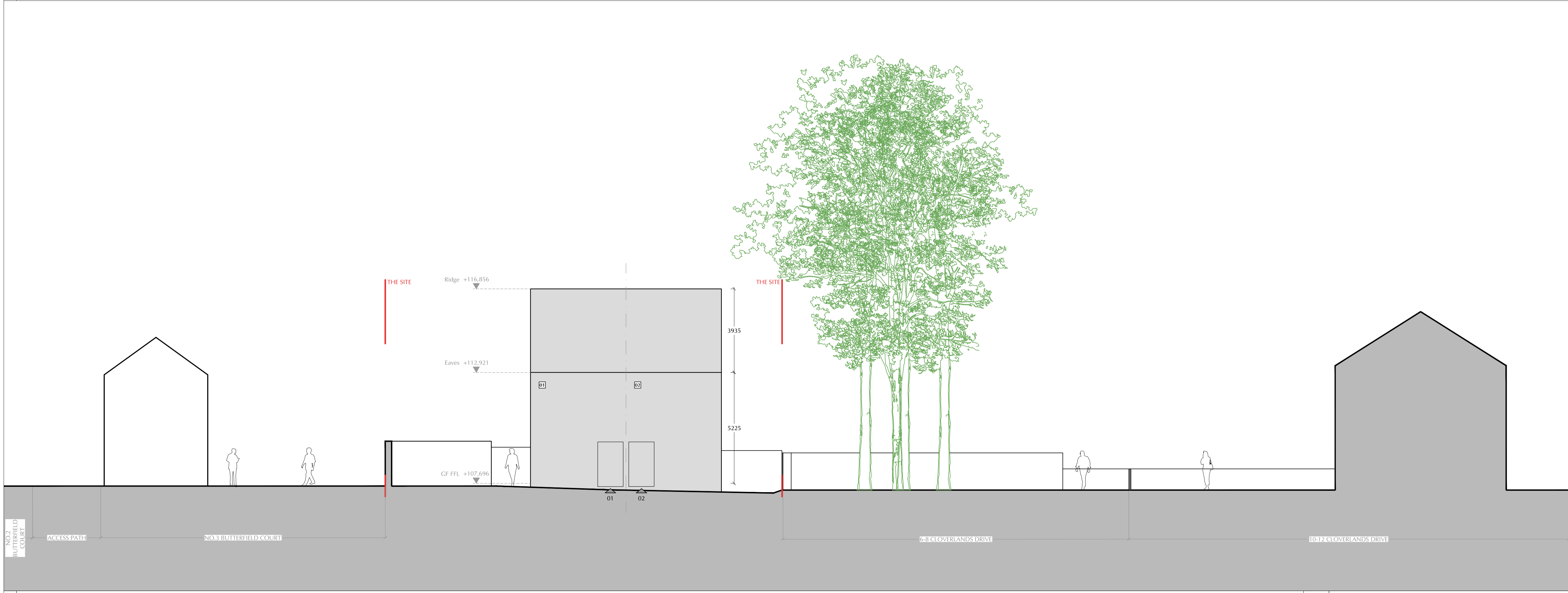
02 Street Section BB
